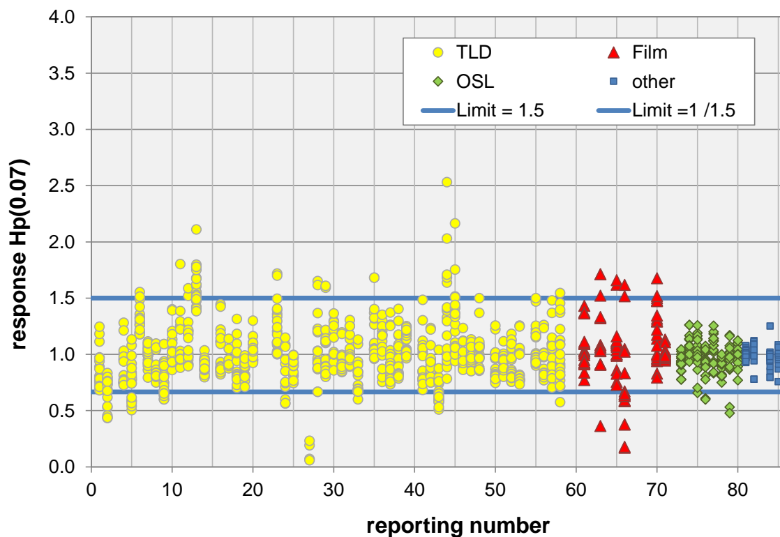
Figure 15: Response values for H_p(10) (top) and H_p(0.07) (bottom) for each individual participant system. Film, TLD, OSL and other systems are represented by triangles, circles, diamonds and squares, respectively.
